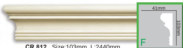
CR 812 Size:103mm L:2440mm
