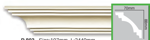
P 803 Size:107mm L:2440mm
