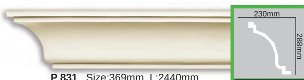
P 831 Size:369mm L:2440mm
