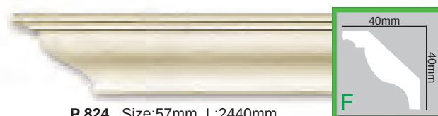
P 824 Size:57mm L:2440mm
