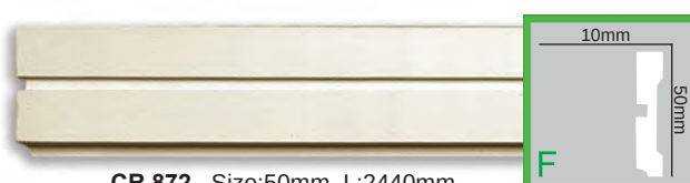
CR 872 Size:50mm L:2440mm
