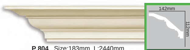
P 804 Size:183mm L:2440mm
