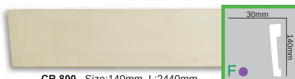
CR 800 Size:140mm L:2440mm
