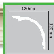
C 791 120x120mm L:2440mm
