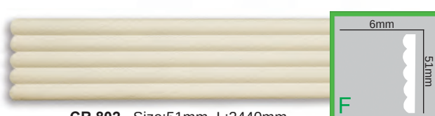
CR 802 Size:51mm L:2440mm
