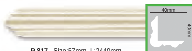
P 817 Size:57mm L:2440mm
