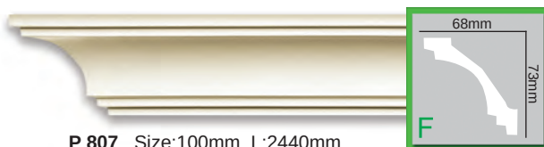
P 807 Size:100mm L:2440mm
