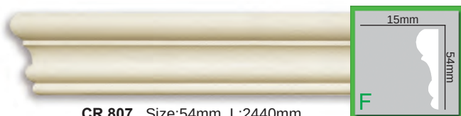
CR 807 Size:54mm L:2440mm
