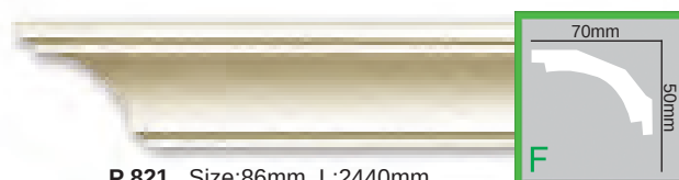
P 821 Size:86mm L:2440mm
