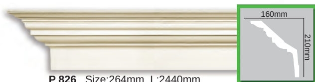
P 826 Size:264mm L:2440mm
