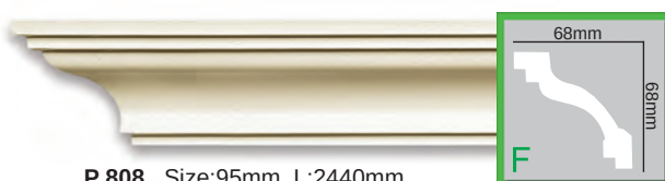
P 808 Size:95mm L:2440mm
