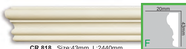
CR 818 Size:43mm L:2440mm
