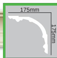
C 756 175×175mm L:2440mm
