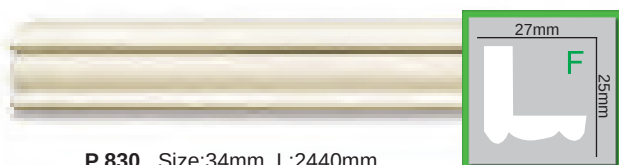
P 830 Size:34mm L:2440mm
