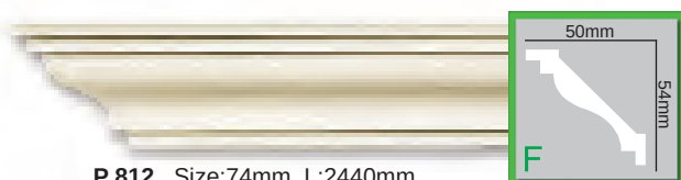
P 812 Size:74mm L:2440mm
